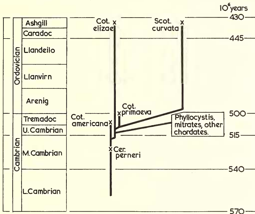
TEXT-FIG. 1. The age and phylogeny of forms mentioned in the text.
